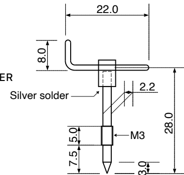
GAS CONTROL VALVE
