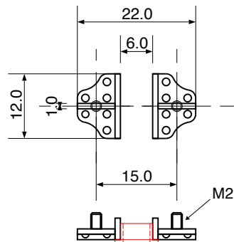
AXLE BOX SUPPORT
