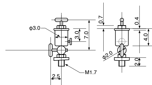
CYLINDER LUBRICATOR
