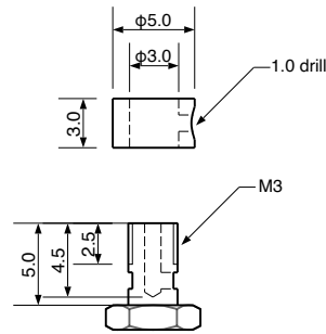
BANJO BOLT
