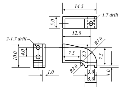
SLIDE BAR BRACKET (R&L.HAND)
