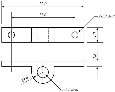
SUSPENSION PIVOT BLOCK ×2
